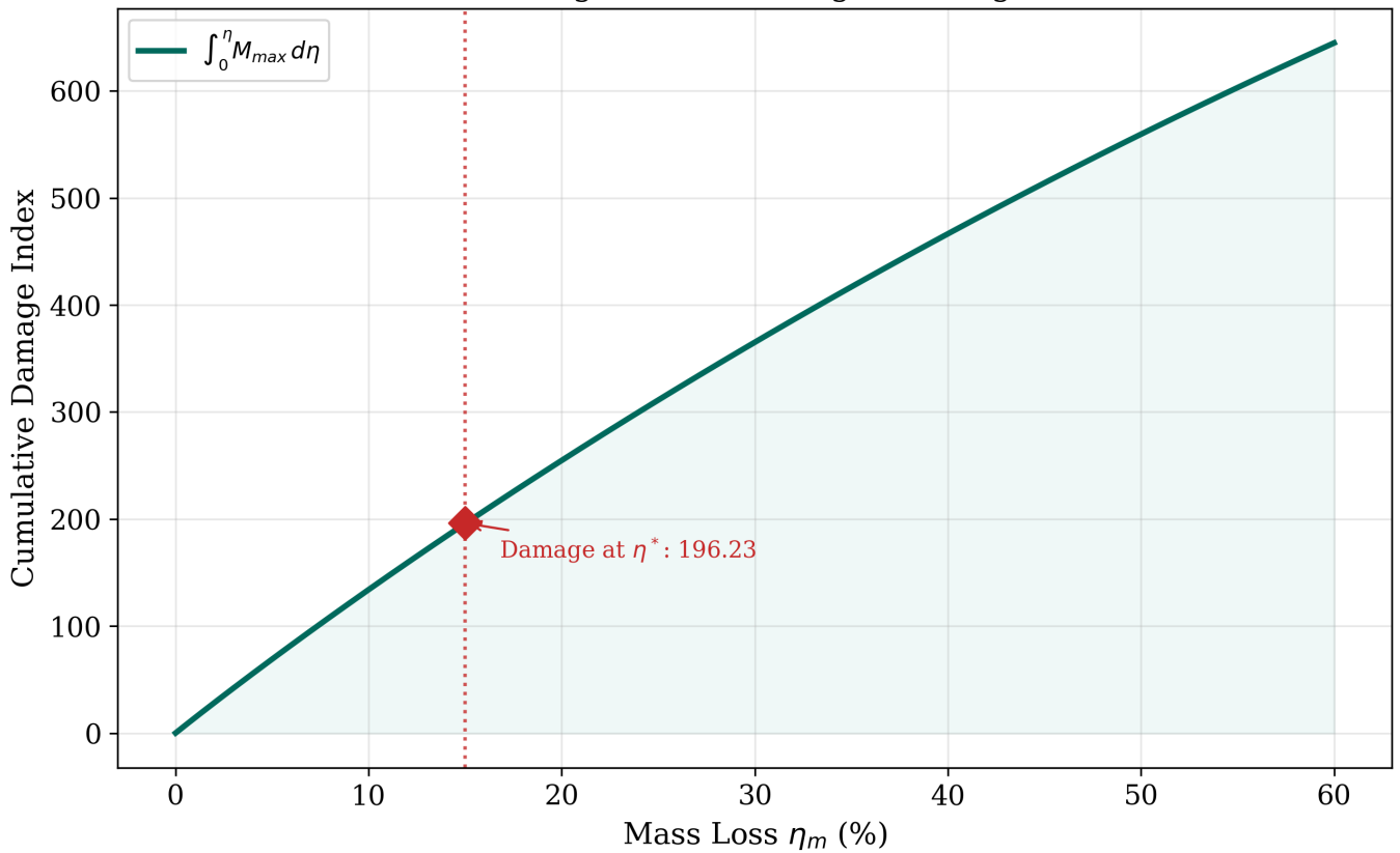
Fig P4 Cumulative Damage
